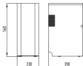
Side cooling unit
